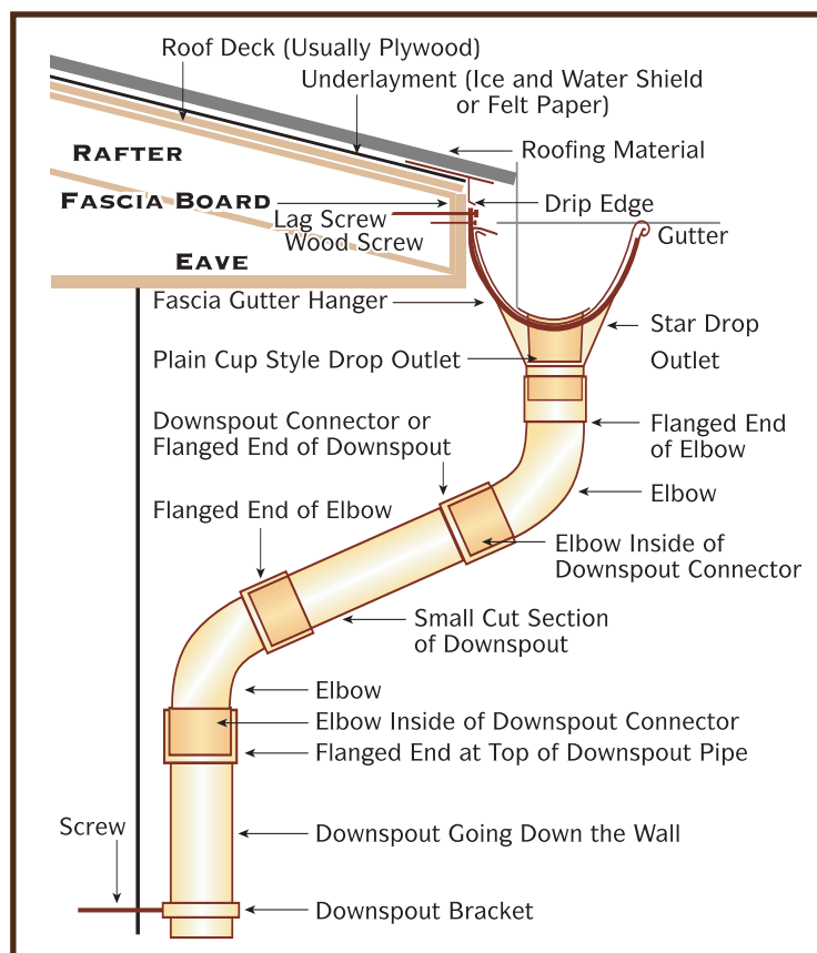
Basic Installation Of The World Gutter System Components
